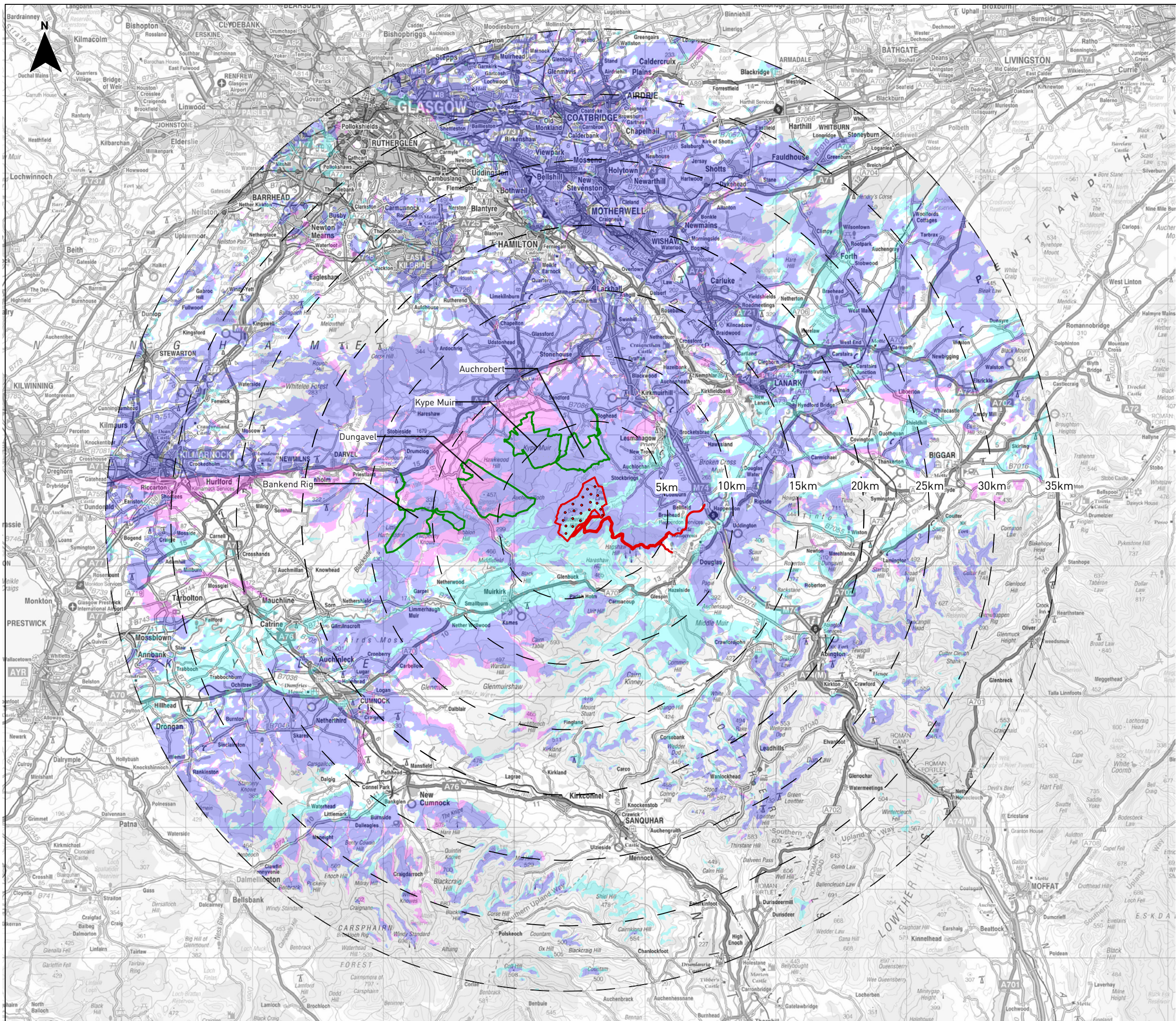
Cumberhead West Wind Farm Environmental Impact Assessment Report Figure 6.28 - Cumulative ZTV with Auchrobert, Kype Muir, Dungavel and Bankend Rig
